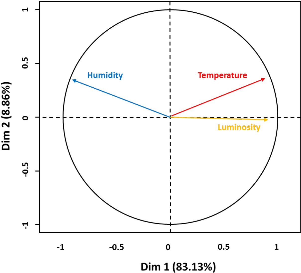
PCA1 (climatic factors)
