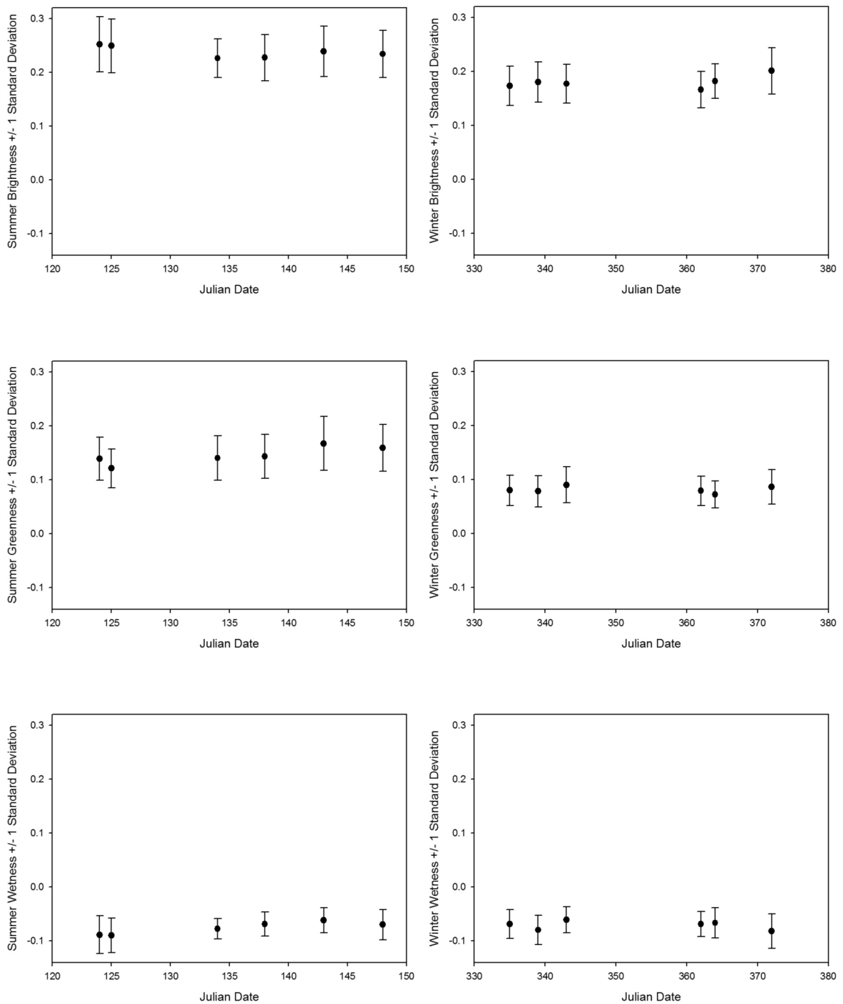
Figure S1. Phenological trends in Tassel-Capped environmental indices from 1985–2007.
