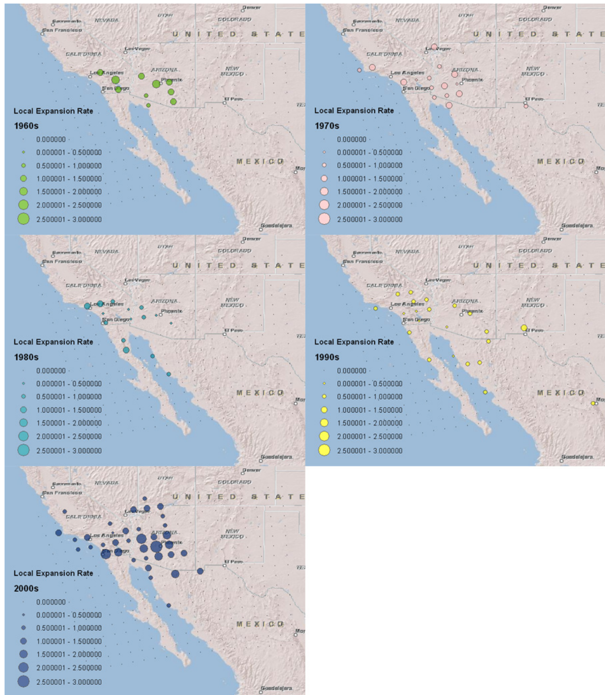
Figure A6. Hotspots of local expansion from 1960s to 2000s. Each circle centers on the geographic center of each 100 x 100km square cell. The size of the circle indicates the rate of expansion (in natural log scale).
